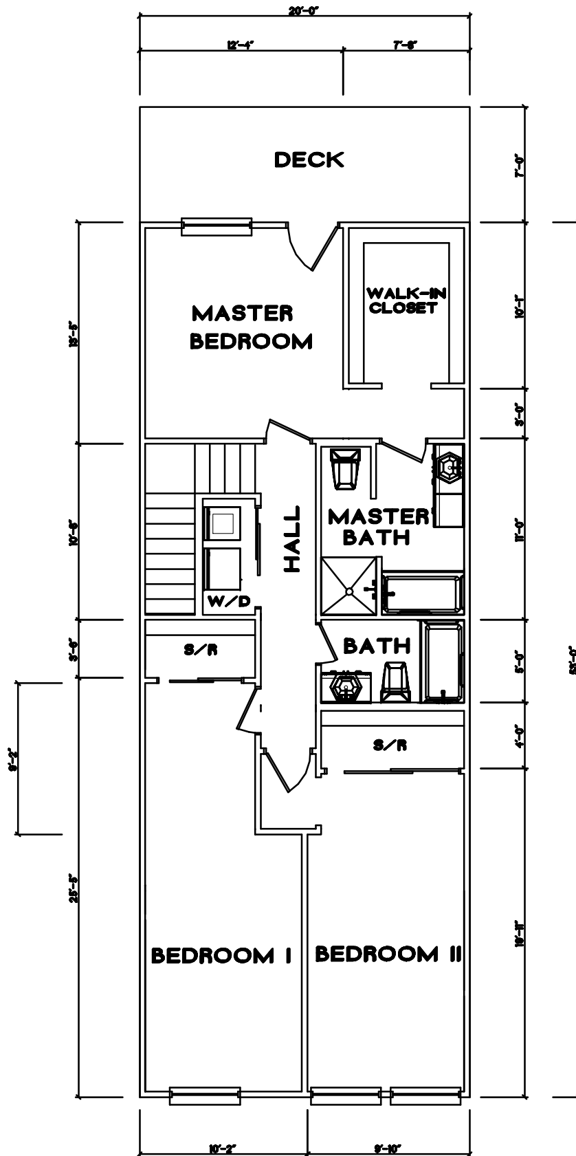
the "Texan" SECOND FLOOR PLAN MODEL B
