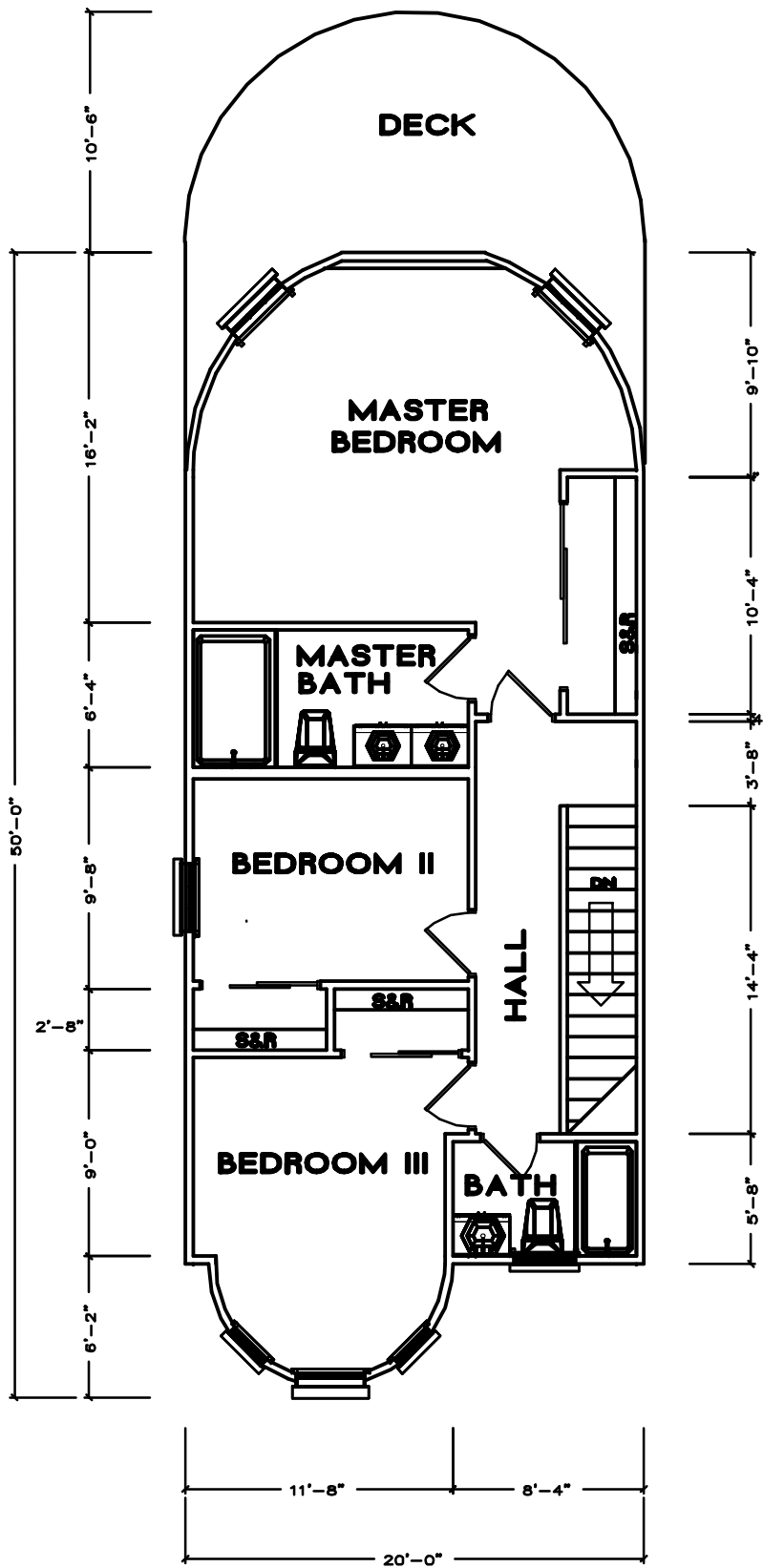
SECOND FLOOR PLAN MODEL A
